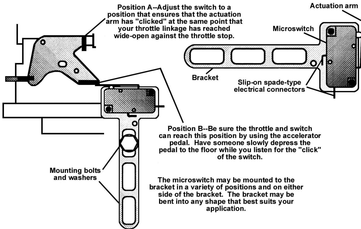
Figure 4 Microswitch Mounting
