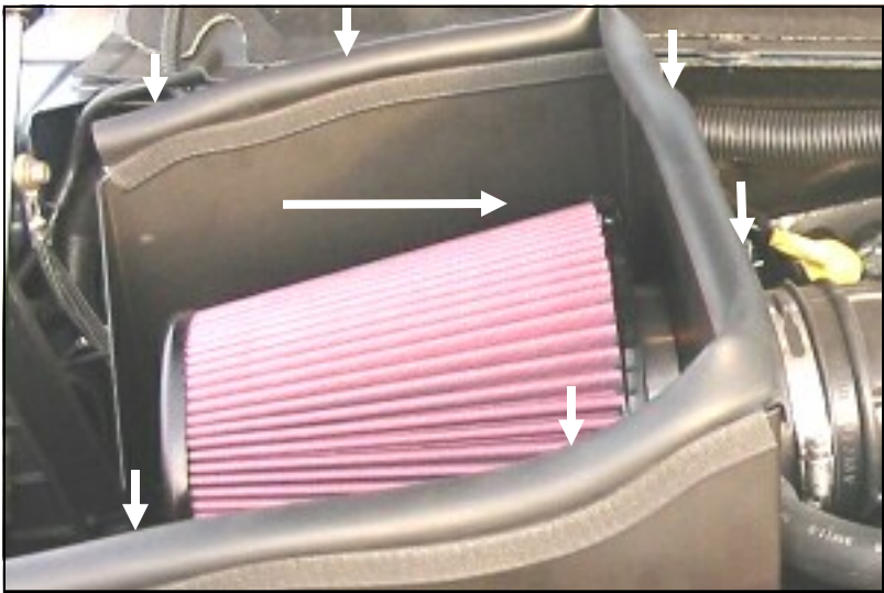
7. Mount the Airaid Premium Filter (#1) onto the CAD and tighten the hose clamp. Install the weather strip (#3) onto the top of the CAD as shown. (Note: start at one end and work your way around to the other to insure proper alignment of the weather strip).
